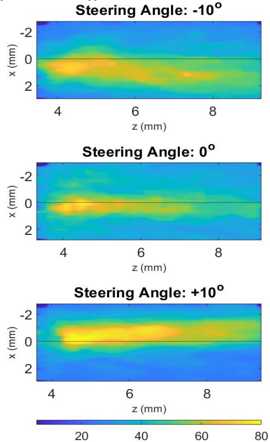
Figure 6: Acoustic pressure map (in kPa) in the XZ-plane of 13 \times 13 element passive layer-free curved PMUT array driven at 22 V, 2 cycles, 2 MHz of sine wave, steer angle = -10^\circ , 0^\circ , +10^\circ .
