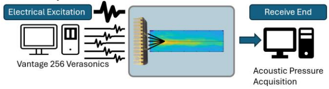
Figure 5: The schematic of acoustic pressure characterization using a hydrophone and the Vantage 256 Verasonics ultrasound data acquisition system.
