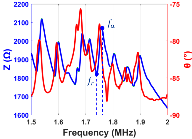
Figure 4: Impedance measurement of element #3
