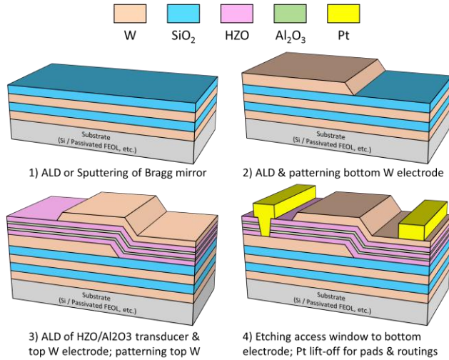
Fig. 3: Four-step fabrication process for creation of CMOS-BEOL compatible, high k_r^2 Q , HZO transduced, SMR resonators.
