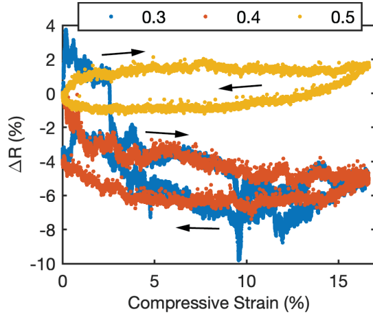
Figure 4: DefeXtiles response to compression and buckling. A representative sample of each EM is included.
