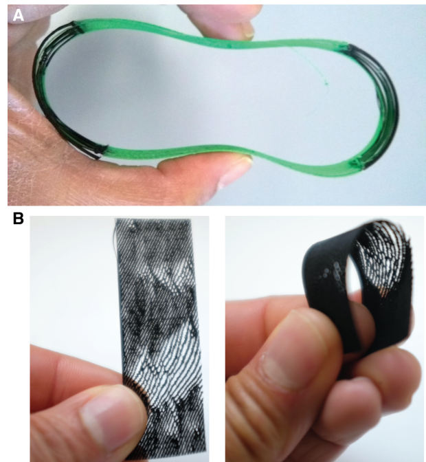
Figure 1: Photographs of defeXtiles samples. (a) A multi-material band with standard PLA (green) and conductive PLA (black). (b) A conductive sample with extrusion multiplier (EM) = 0.4.
