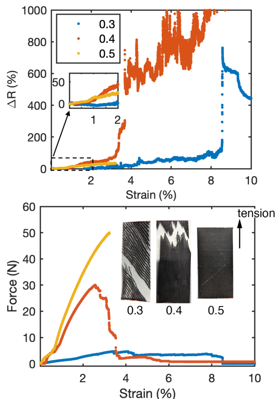
Figure 3: Resistance (top) and force response (bottom) to tension during one cycle of loading to failure. A representative sample of each EM is included.
