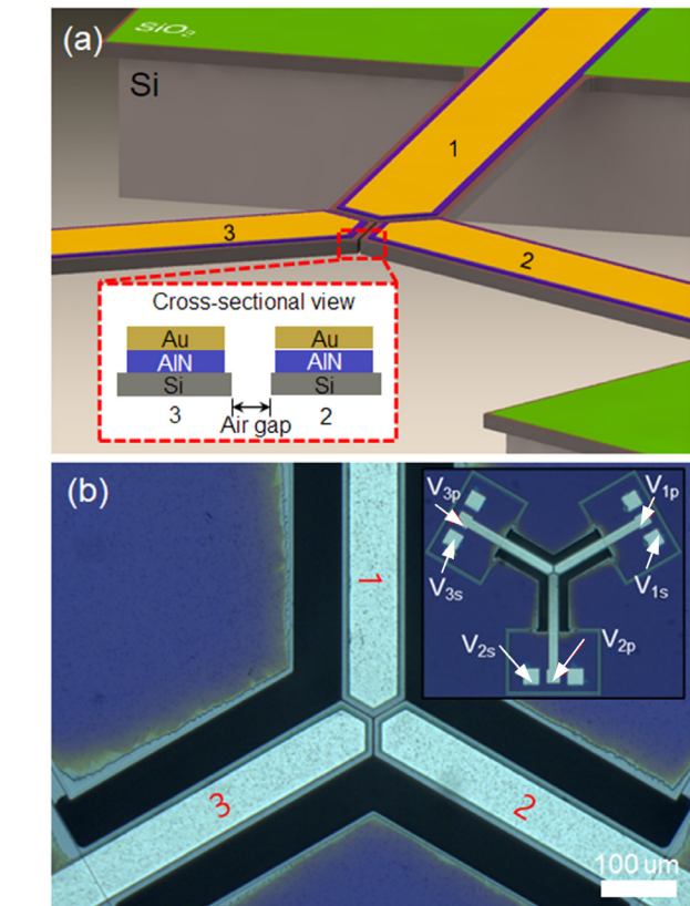
Figure 1: (a) Diagram of a 3-resonator closed-chain array. Inset: Cross-section of device layers. (b) Optical micrograph of a fabricated array. Inset: Electrical connections for the drive and coupling voltages.
