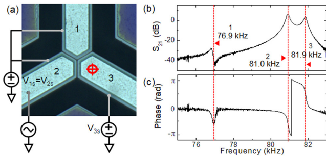
Figure 4: (a) Second coupling scheme for the array. Resonator 2 is driven with an AC signal while the same bias voltage is applied to the silicon layers of resonators 1 and 2. An independent voltage is applied to resonator 3. (b) Representative amplitude and (c) phase responses measured on resonator 3 with the interferometer (location indicated by the red cross in (a)). V_{1s} = 0 V, V_{2s} = 0 V.
