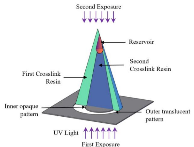
Figure 1. Conceptual drawing of the hollow-well microneedle.
