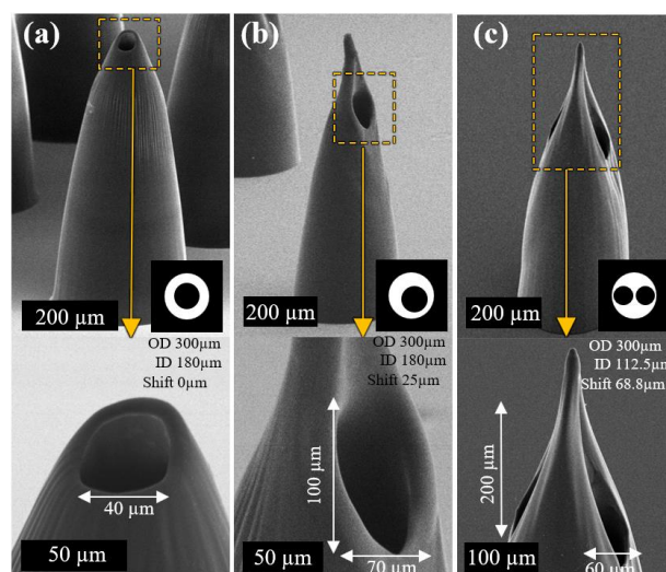
Figure 3. SEM images of the hollow-well microneedles fabricated with three photomask designs. (a) Center-well, (b) side-well, (c) dual-well (upper) and close-up (lower).
