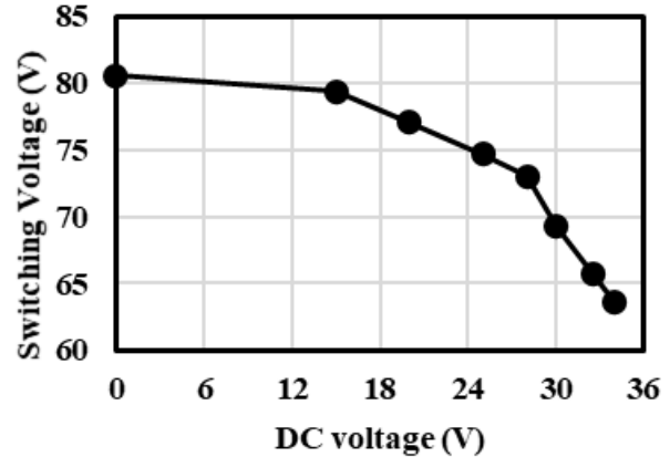
Figure 8: The measured switching voltage for different ovenization voltages. Application of larger ovenization voltage results in significant drop in coercive field and resonator switching voltage.
