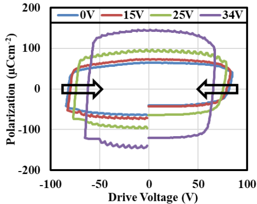
Figure 6: Evolution of the PV loop for bottom \text{Sc}_{0.28}\text{Al}_{0.72}\text{N} layer, for different ovenization voltage (applied across top electrode). The large drop in coercive voltage with increasing ovenization voltage is evident. The apparent increase in polarization is due to increase in leakage current at higher temperatures.
