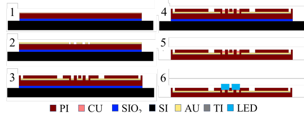
Fig. 2. Fabrication process flow of the opto-electro array.
