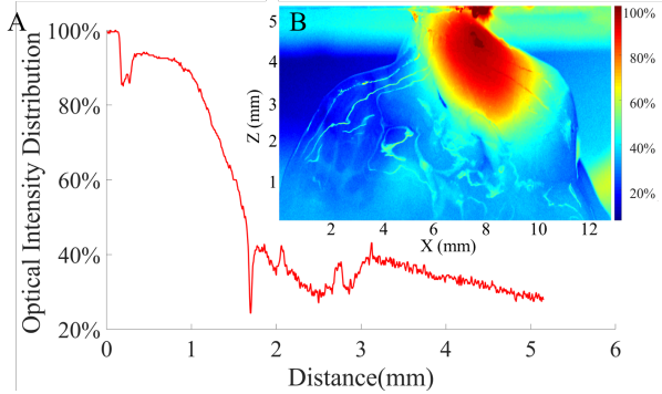
Fig. 4. (A) Optical intensity distribution measured from the \mu -LED to the surrounding mouse brain. (B) Photo image of the optical intensity distribution around the \mu -LED in the mouse brain (input power = 15\text{mW} /optical power = 3.85\text{mW} )
