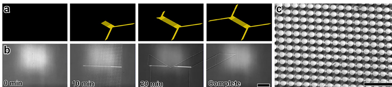
Figure 2: Fabrication Results. (a,b) Sequential images of (a) computer-aided manufacturing (CAM) simulations, and (b) the corresponding DLW-based printing process of the mold onto a Si wafer. Scale bar = 250 \mu\text{m} . (c) SEM micrograph of print results. Scale bar = 200 \mu\text{m} .
