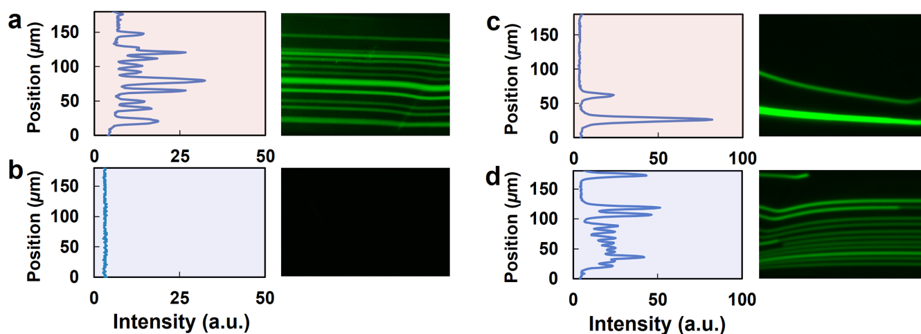
Figure 4: Quantified fluorescence intensity results (left) and corresponding fluorescence micrographs (right) associated with the (a,b) inlets and (c,d) outlets for the (a,c) microparticle suspension fluid and the (b,d) surrogate 'reactant' fluid.
