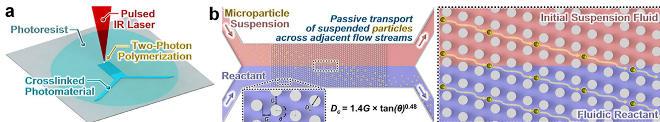
Figure 1: Conceptual illustrations of a “Direct Laser Writing (DLW)”-based “Deterministic Lateral Displacement (DLD)” array continuous-flow microfluidic particle reactor. (a) DLW of the microfluidic system master mold onto a Si wafer. (b) Microfluidic system overview. Suspended microparticles are inputted via the top left channel, enter the DLD array to be passively guided into the distinct, adjacent “reactant” flow stream, and outputted via the bottom right channel. The critical (i.e., minimum) diameter ( D_c ) of suspended particles that can be transported is based on the gap spacing ( G ) and the angle of the array ( \theta ) with respect to the primary flow direction.
