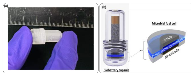
Figure 2: (a) Images of the assembled capsules and (b) the MFC configuration integrated in the capsule.
