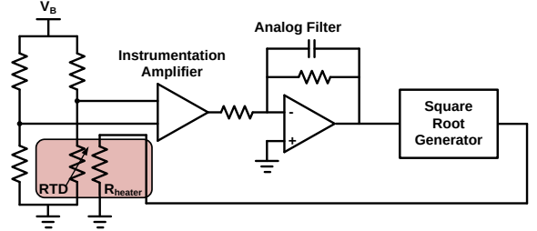
Figure 4: Circuit schematic of the resistive temperature detector (RTD) interface and analog oven-control system.
