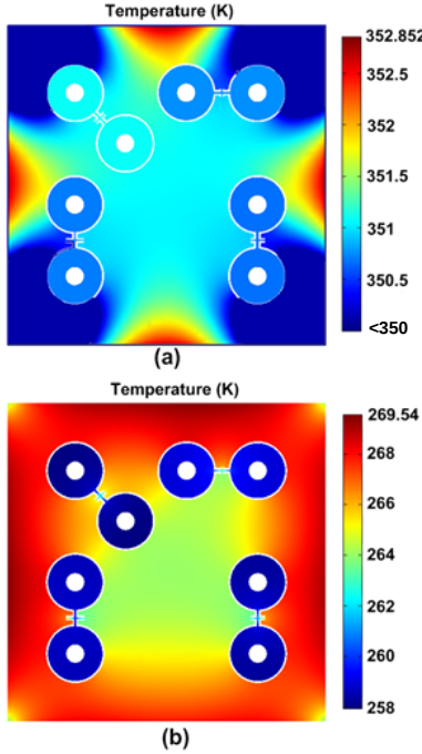
Figure 3: Temperature distribution within the active area when 4.3 mW of power is applied to the heater at an external temperature of 233 K: (a) only considering conduction heat transfer; (b) considering heat conduction, convection, and radiation.
